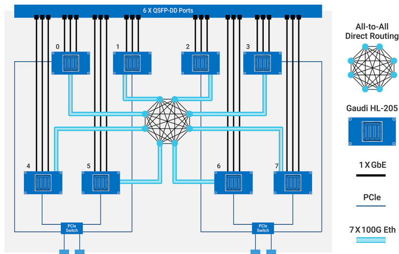
HLS-1 Block Diagram
